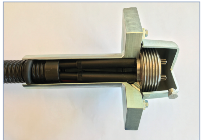
Example of a strand anchor head (permanent)
