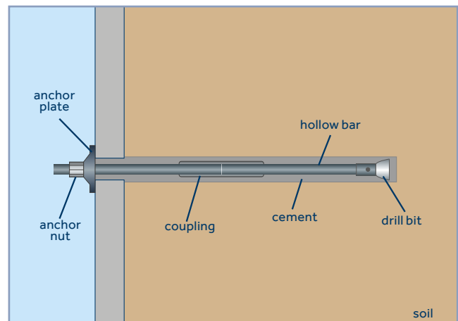
Soil nail with hollow bar
