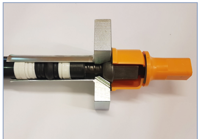
Example of a bar anchor head (permanent)
